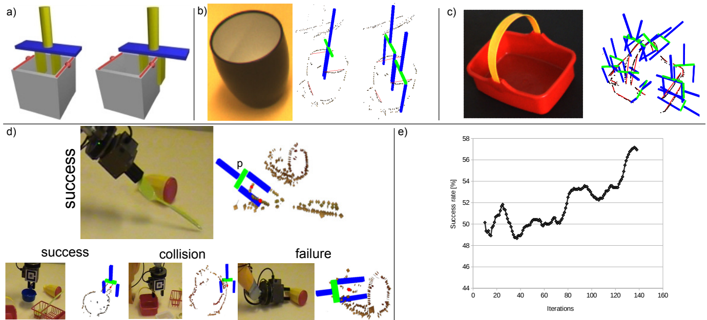
Fig. 6. Grasping reflex. a) Based on two coplanar and co-colour visual contours certain grasps are predicted by a specific contour pair. b) Concrete situation and the grasps predicted by a specific contour pair. c) More complex scene and a selection of predicted grasps. d) Results based on real grasping attempts stored in the episodic buffer. The gripper pose (p), the position of the centres of the two generating contours (visualised as red dots here) as well as the evaluation result are stored. e) The success rate after learning versus the increase of the learning set.
